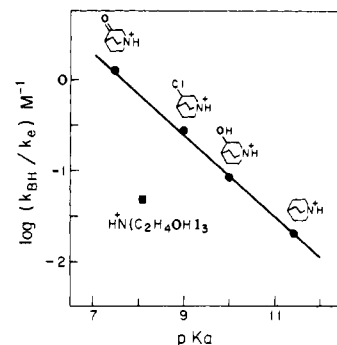
Figure 6. The Brønsted plot for general acid catalysis of enediolate protonation at C-1. Reaction was at 37 °C, ionic strength of 1.0 (KCl), and pH 8.1 (0.2 M triethanolamine).
